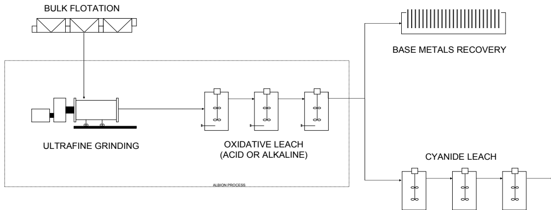
Figure 1 - Albion Process schematic flowsheet
